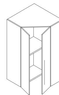
Cabina a 2 ante H 2300/2550/2870 mm L 1300 x L 1300 mm 2 Door walk-in wardrobe H 2300/2550/2870 mm L 1300 x W 1300 mm
